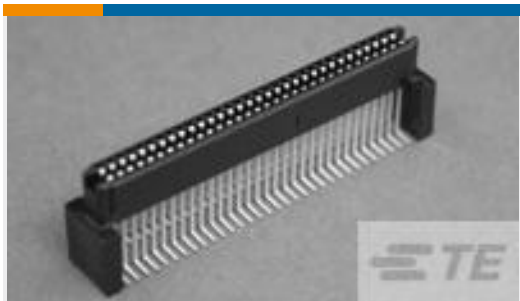
TE 零件编号120524-2 1FHR,84,30A/P,S,N,S14,15
