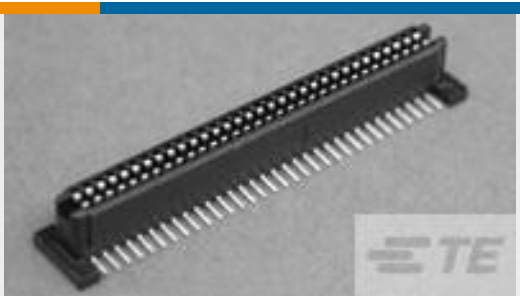
TE 系列/零件编号5120521-1 1FHR,64,30A/S,S,N,S08, 09,10
