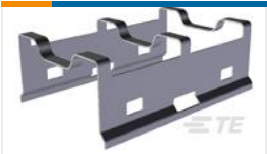
TE 系列/零件编号1489948-2 XFP HEAT SINK CLIP, PLATED
